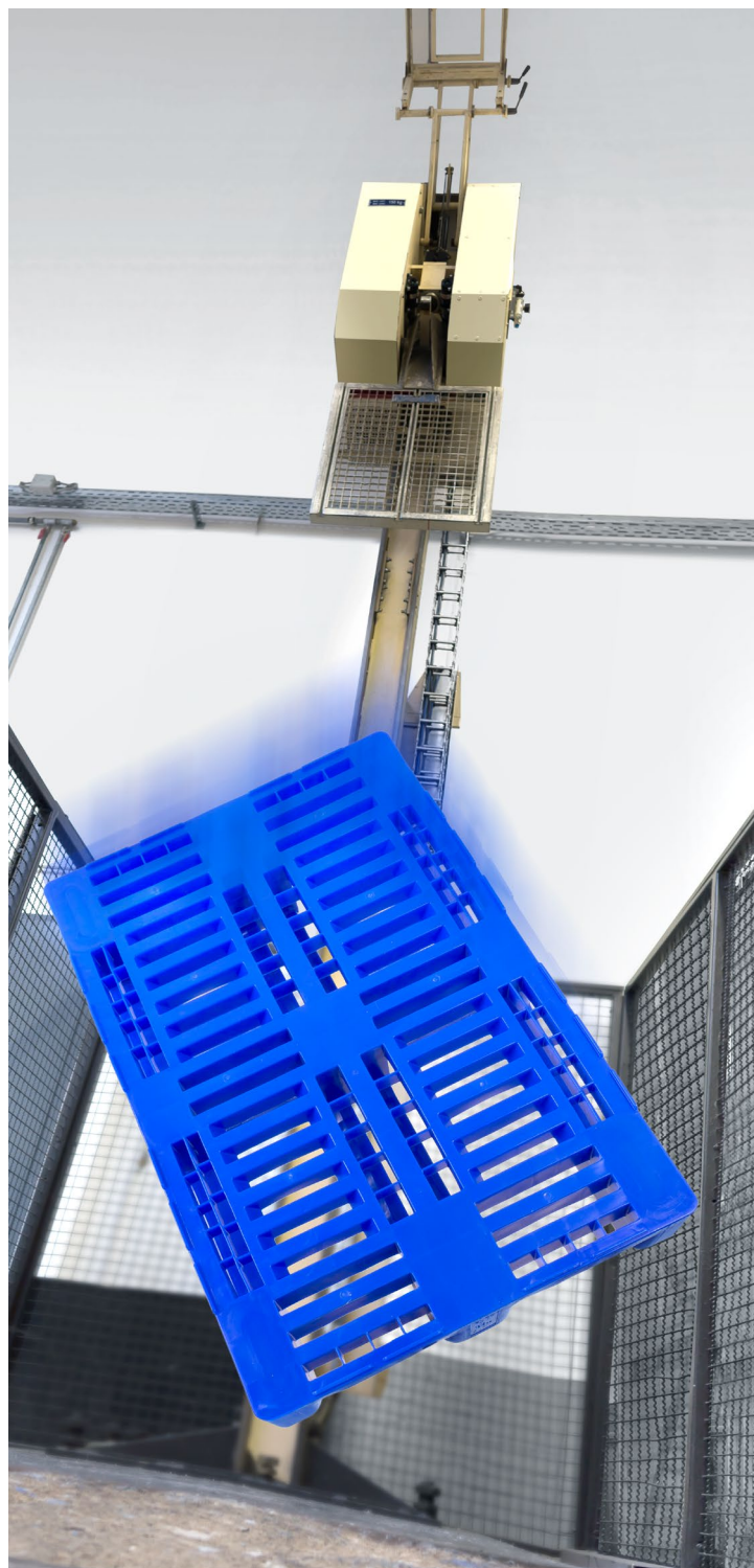
Corner drop test
